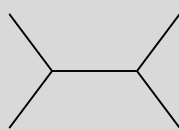
s-channel
